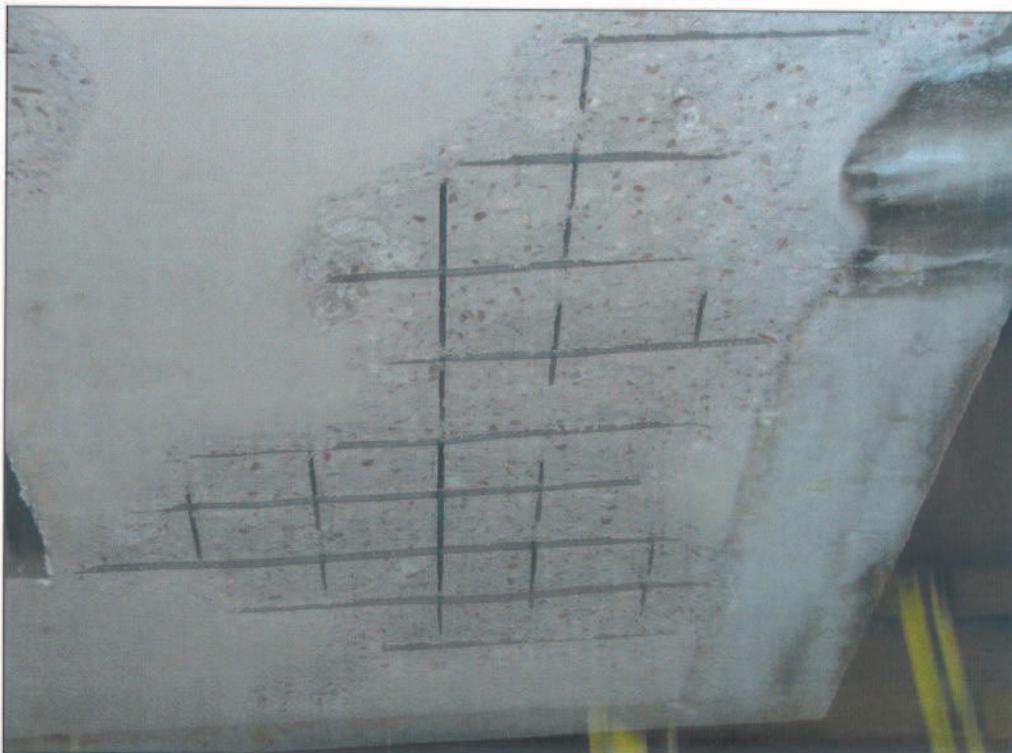
ES of supporting structure – reinforced concrete panel after the finished test of fire resistance
