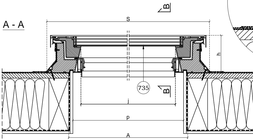
735-DRF DU8 FAKRO flat access roof light opened manually, glazing unit DU8
