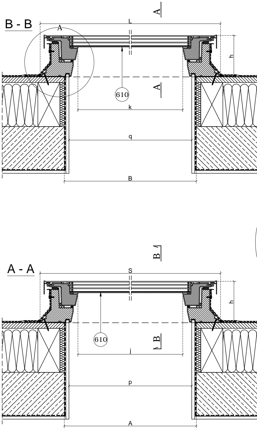
610-DXF DU8 Flat Roof Window, non-opened, Flat, DU8 glazing unit
