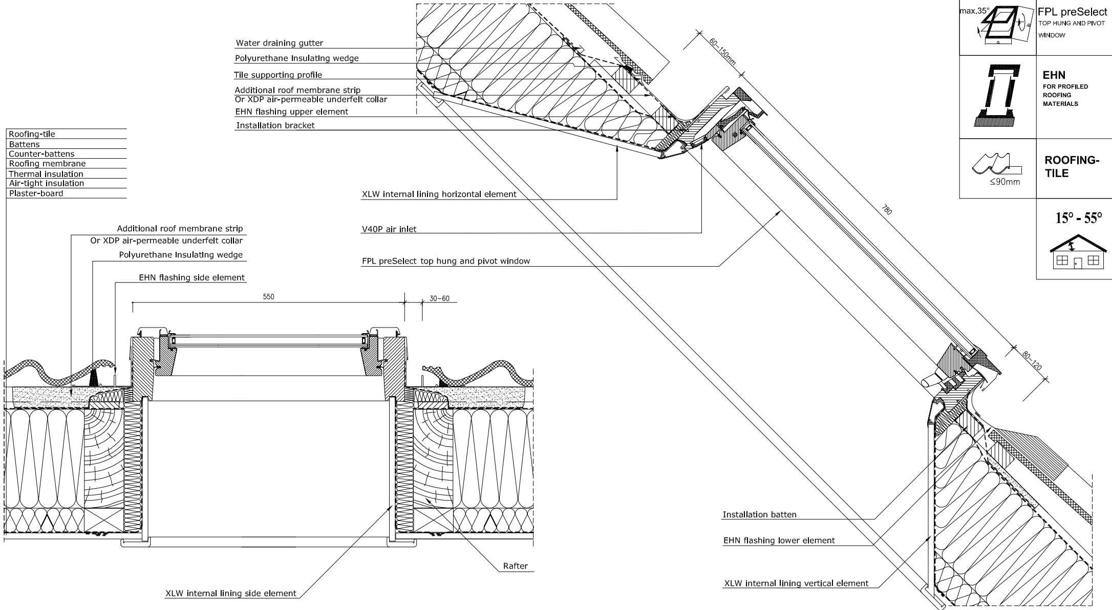
Vertical and horizontal cross-section: FPL preSelect top hung and pivot window with EHN flashing for profiled roofing materials
